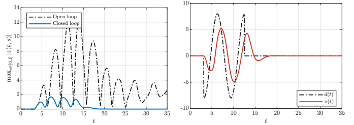
(a) Spatial-amplitude comparison (b) Disturbance and control effort Fig. 7. Time-domain data corresponding to Fig. 6: (a) the spatial peak \max_{s \in [0,1]} |\mathbf{z}(t, s)| and (b) the injected disturbance d(t) and boundary control effort x(t) .
